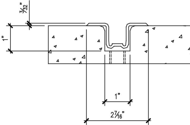
Recessed Flush Hat
