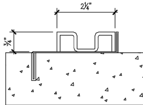
Surface Mount
