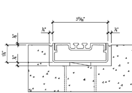
Tank Sill
