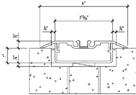
Tank Sill with Ramps
