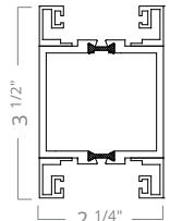
Standard Mullion
