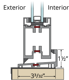
High Performance Outswing Sill 6PSF lab water performance 4PSF field water performance
