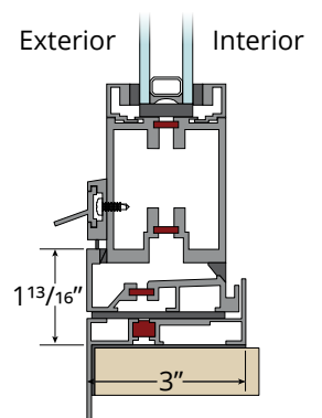
High Performance Inswing Sill with Thermal Sill Pan 4PSF lab water performance 2.67PSF field water performance
