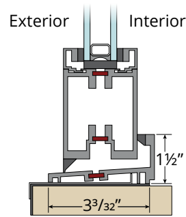
High Performance Outswing Sill 10PSF lab water performance 6.67PSF field water performance
