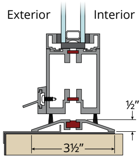
ADA Sill Limited/no water performance ADA compliant
