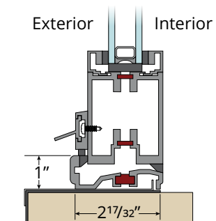
Standard Inswing Sill Limited/no water performance
