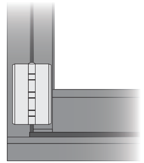
Extra Narrow G3 Panel Vertical and G3LT Narrow Jamb Frame
